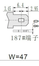
Terminal type (mm):
