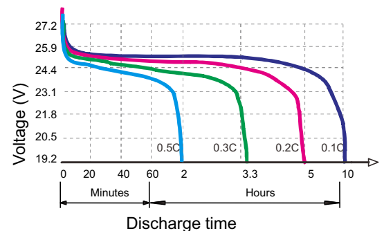
Discharge characteristic at 25°C
